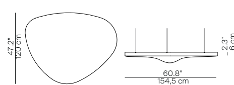
Lamp D71/2 (on/off) D71/2D (DALI) for D71P-D71C-D71P1
